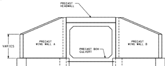
10'0" x 5'0" – Concrete Box Culvert
