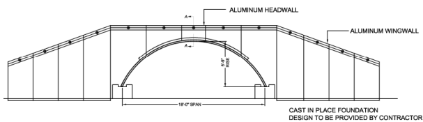
18'0" x 5'9" – Aluminum Structural Plate Arch
